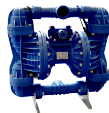
Blue Series - P50BB Polypropylene Body- Santoprene Elastomers- For Acids, Caustics, Chemicals- ATEX M2 Rating
