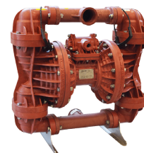
Red Series - P50BR FRAS (Fire Retardant Antistatic) Nylon Body- Hytrel Elastomers- For Explosive Environment- ATEX M1 Rating
